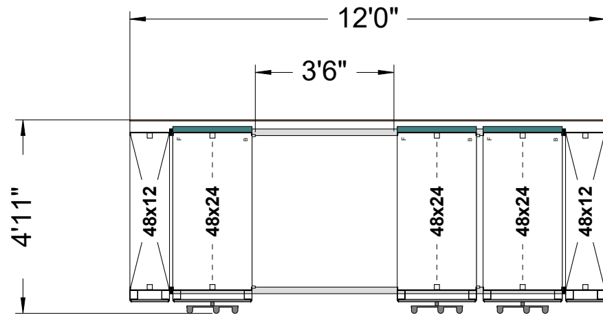
Plan View
