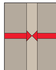
Plan View Full moment welded connection for RT-161 rail
