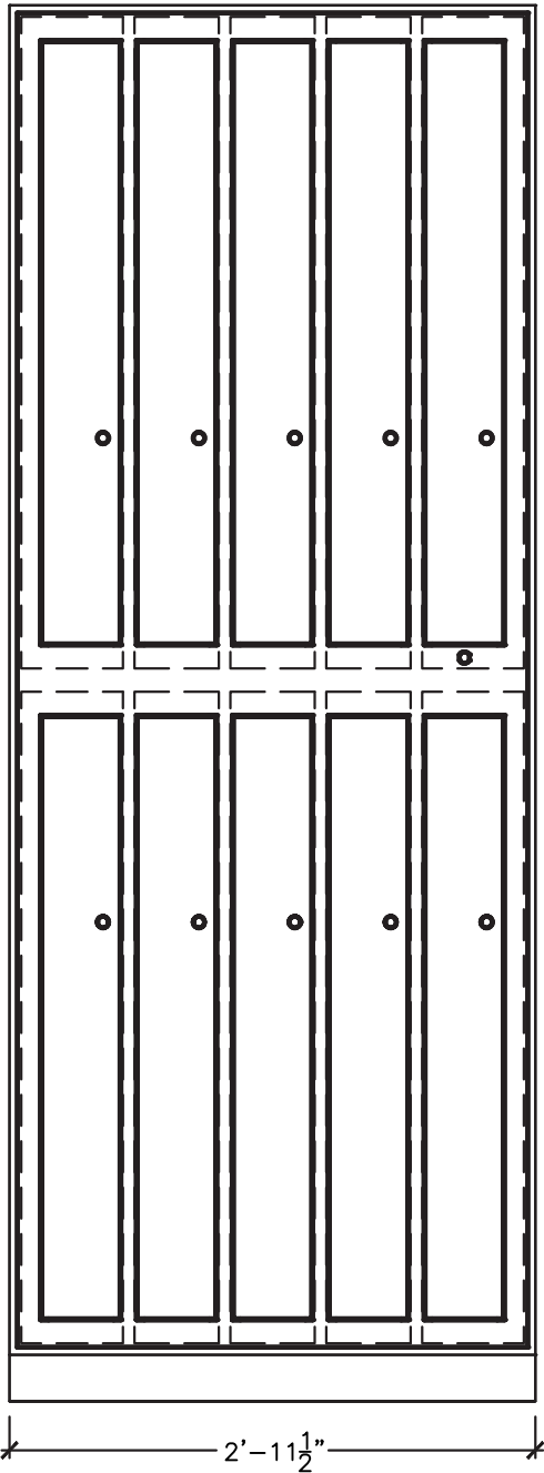
FRONT VIEW
