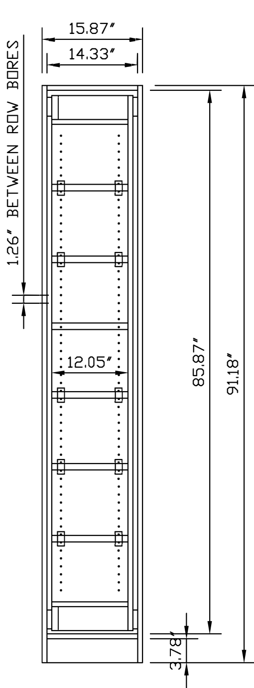
I9500 FRONT VIEW
