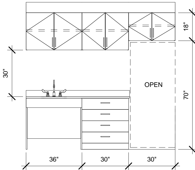
② 8' - Option 6 Front 3/8" = 1'-0"
