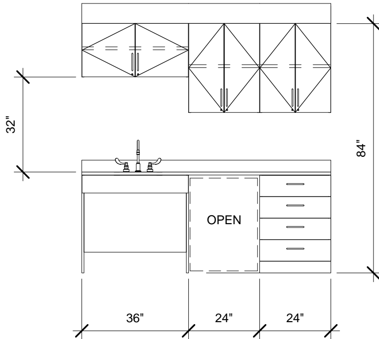
② 7' - Option 2 Front 3/8" = 1'-0"
