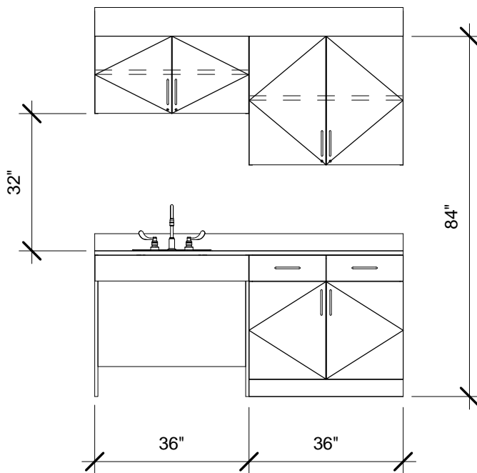
② 6' - Option 2 Front 3/8" = 1'-0"
