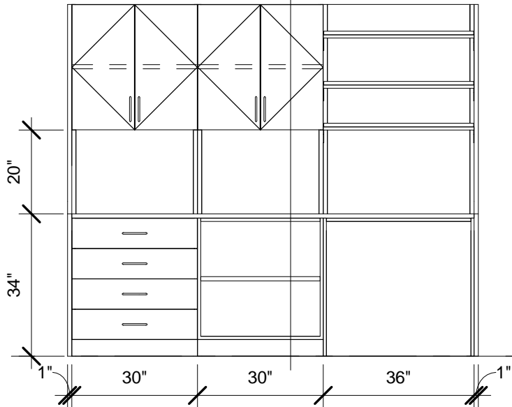
② 8' - Option 4 Front 3/8" = 1'-0"
