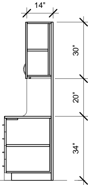
③ 8' - Option 4 Section 3/8" = 1'-0"
