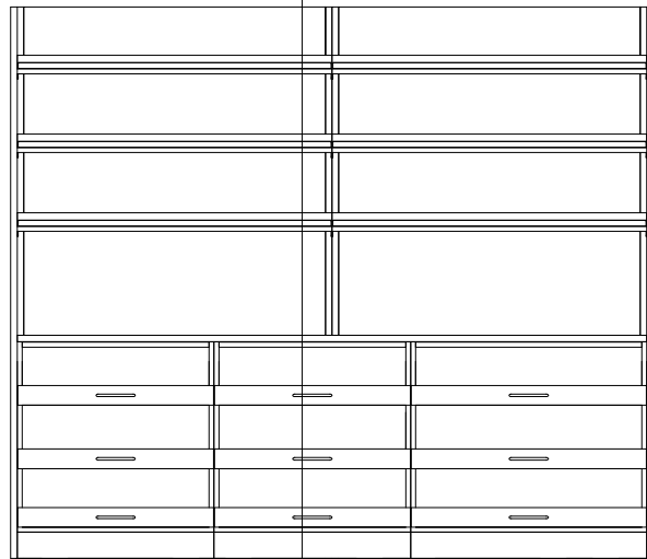
② 8' - Option 2 Front 3/8" = 1'-0"
