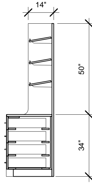
③ 7' - Option 5 Section 3/8" = 1'-0"
