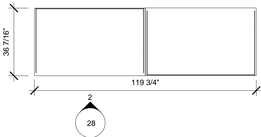
1 10' Option 2 - Plan 3/8" = 1'-0"
