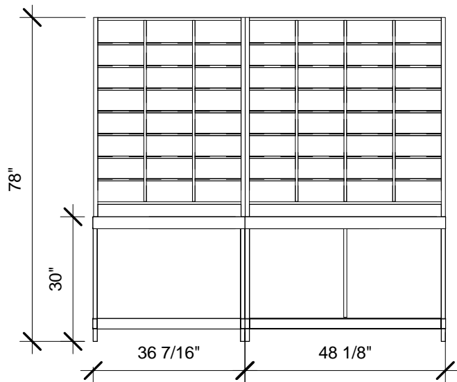
2 7' Option 1 - Front 3/8" = 1'-0"
