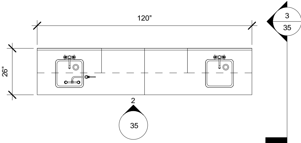
① 10' - Option 5 3/8" = 1'-0"
