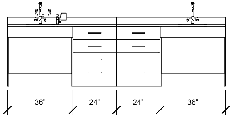
② 10' - Option 5 3/8" = 1'-0"
