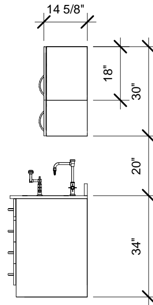
③ 10' - Option 5 3/8" = 1'-0"
