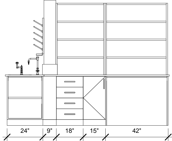
③ 9' - Option 2-B 3/8" = 1'-0"
