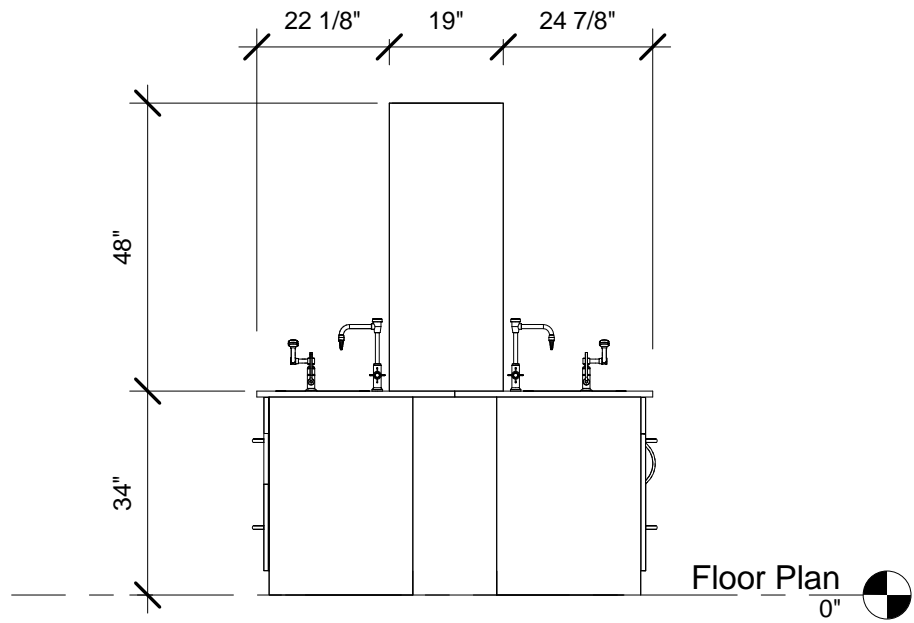
① 7' - Option 2 \frac{3}{8}'' = 1'-0''
