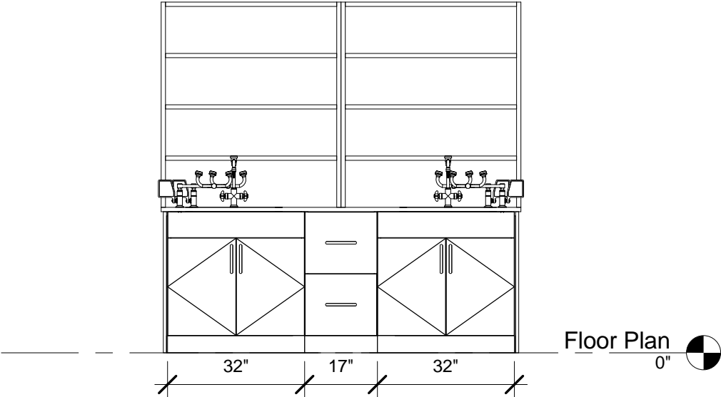
3 7' - Option 2-B 3/8" = 1'-0"
