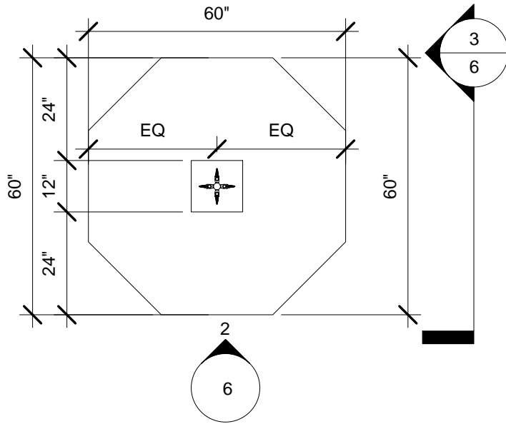
1 5' - Option 6 3/8" = 1'-0"
