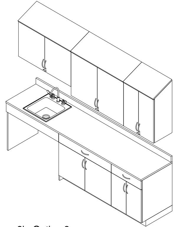
④ 9' - Option 6
