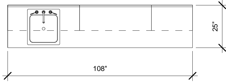
① 09' - Option 6 3/8" = 1'-0"
