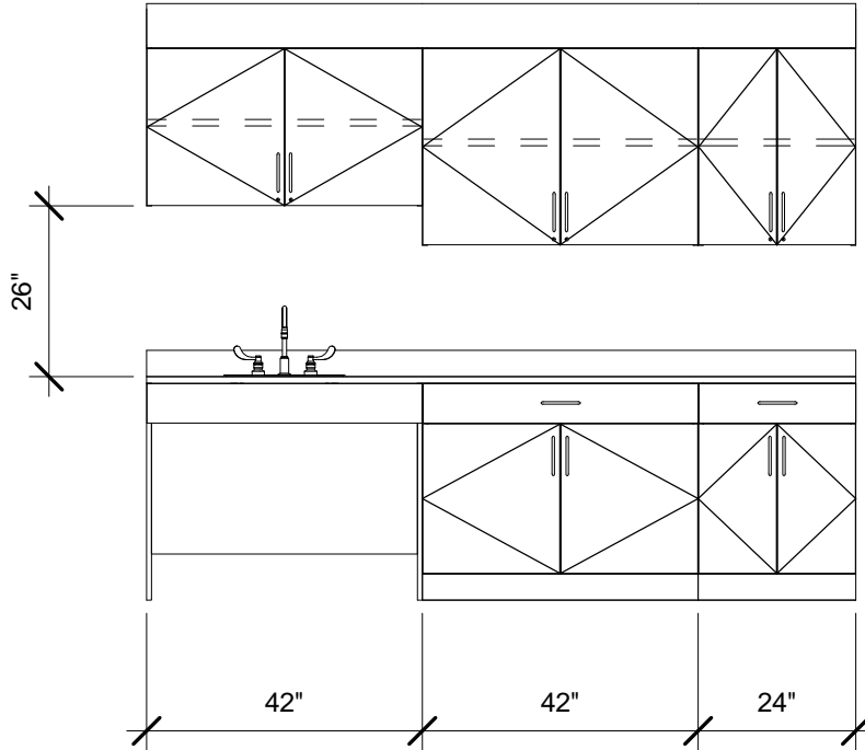
① 09' - Option 6 3/8" = 1'-0"
