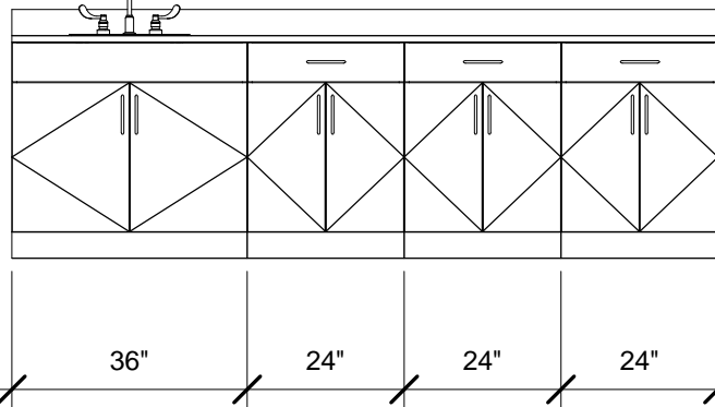
② 9' - Option 3 Front 3/8" = 1'-0"
