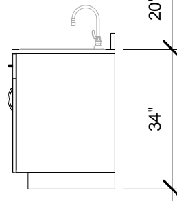
③ 9' - Option 3 Side 3/8" = 1'-0"
