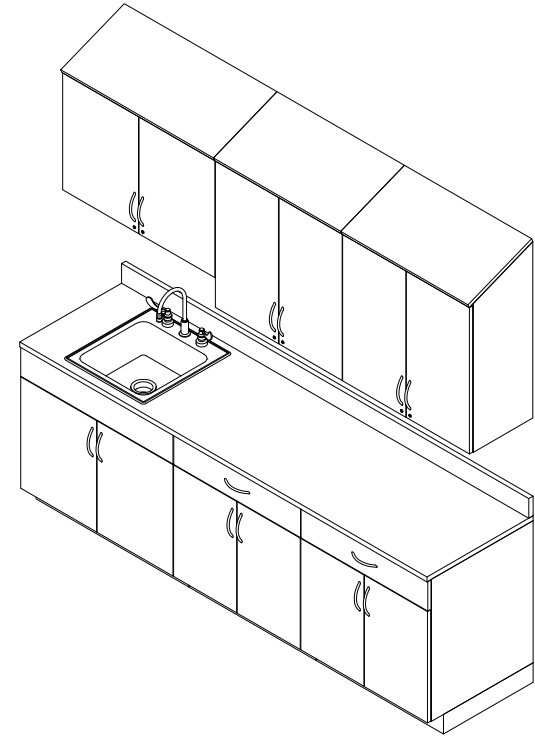
④ 8' - Option 3
