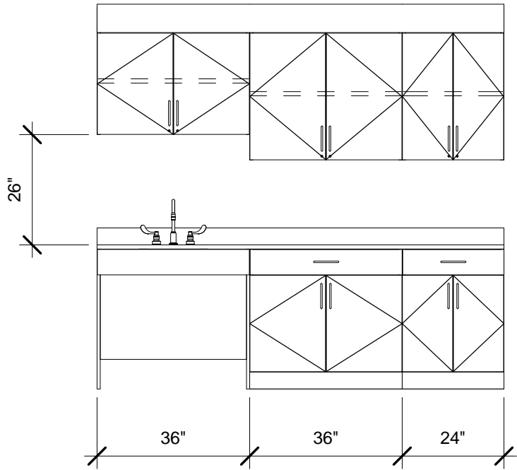
② 8' - Option 2 Front 3/8" = 1'-0"
