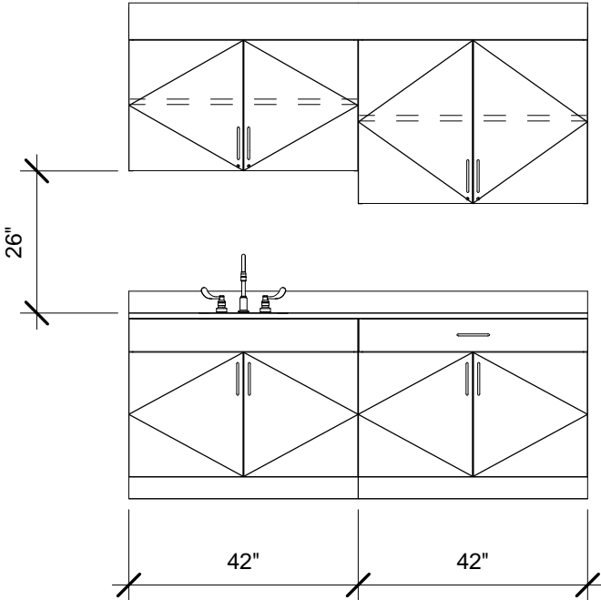
② 7' - Option 1 Front 3/8" = 1'-0"
