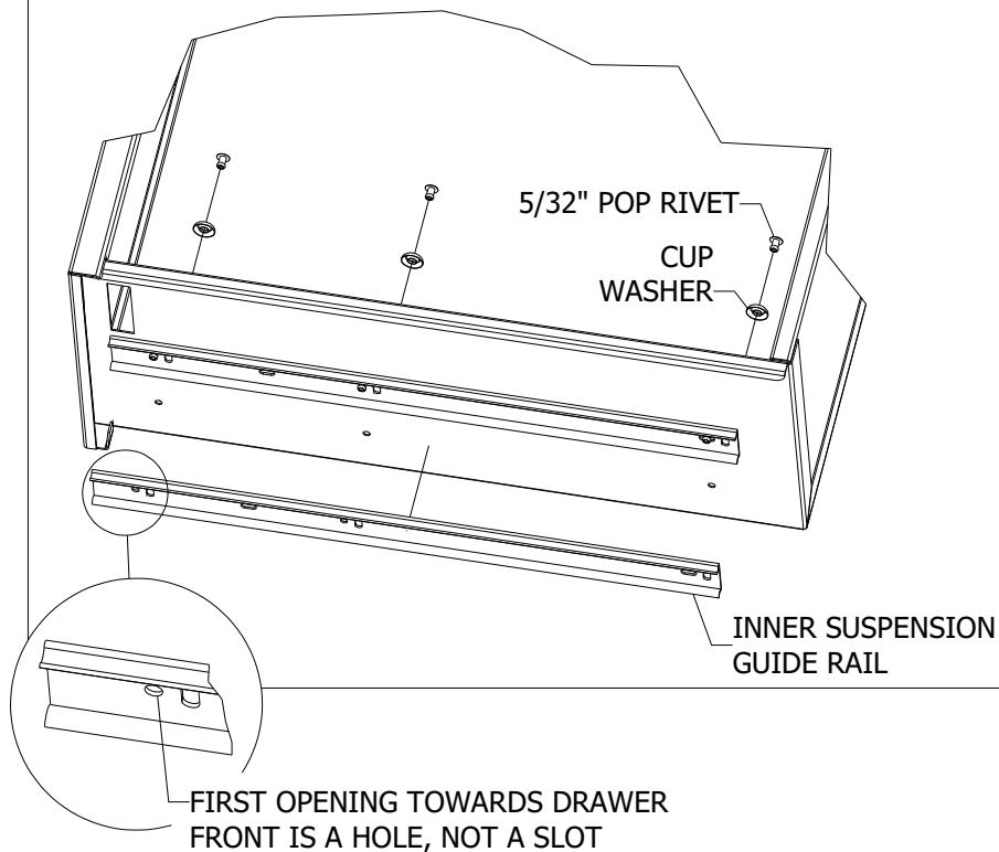
FIGURE A2: INNER SUSPENSION GUIDE RAIL MOUNTING
