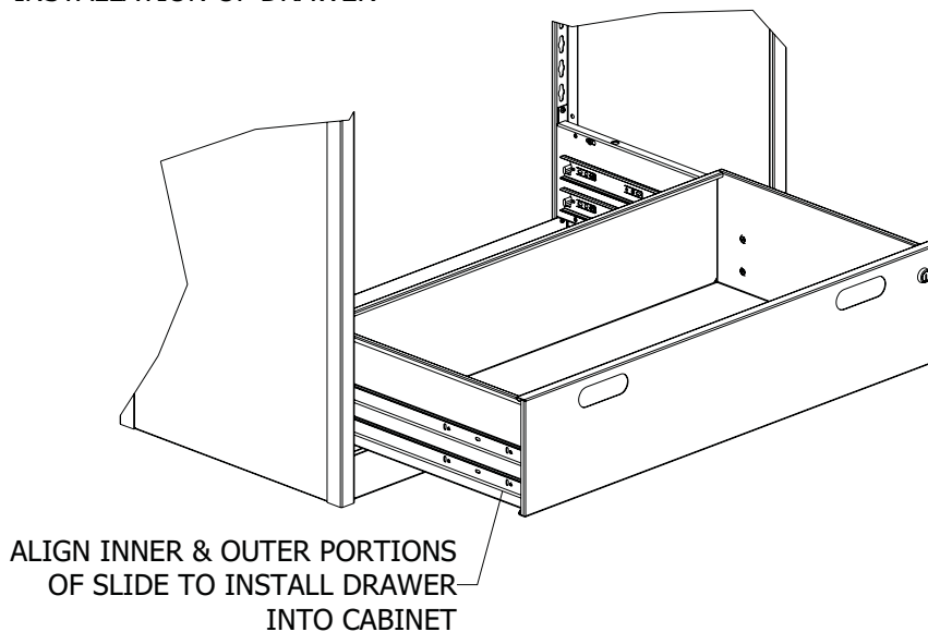
FIGURE I4: INSTALLATION OF DRAWER
