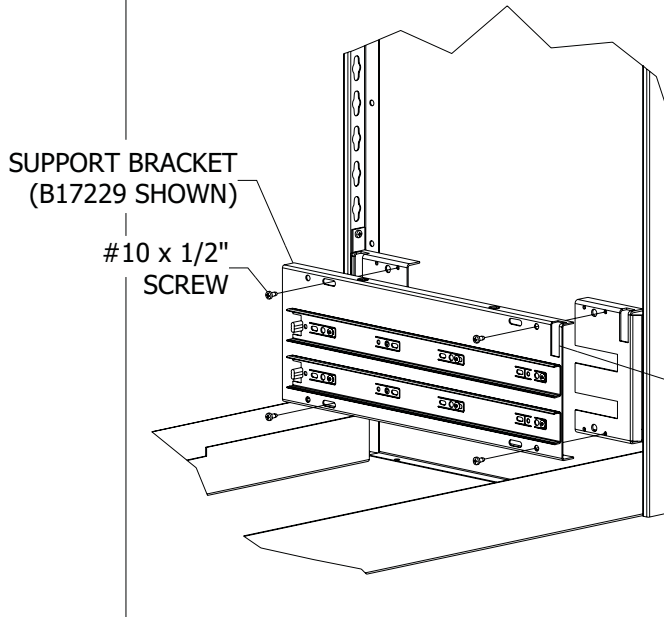
FIGURE I3: SUPPORT BRACKET INSTALLATION
