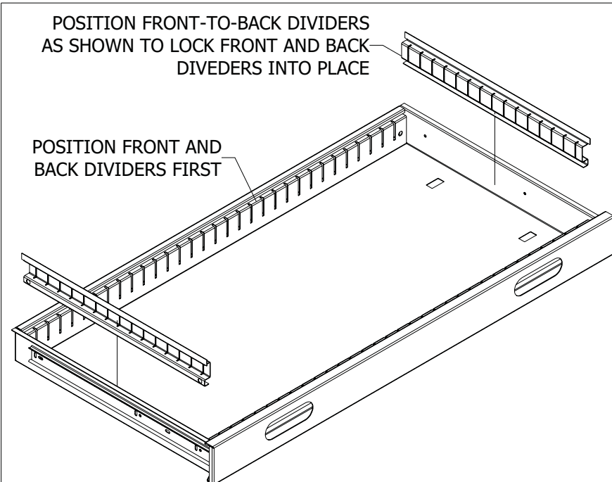
FIGURE I5: MULTI-MEDIA DRAWER DIVIDER INSTALLATION
