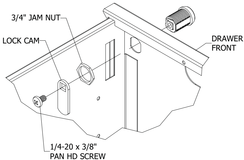
FIGURE A6: ASSEMBLY OF OPTIONAL LOCK COMPONENTS
