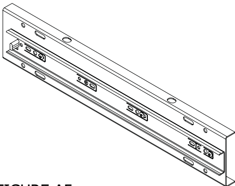
FIGURE A5: C18796 SUPPORT BRACKET
